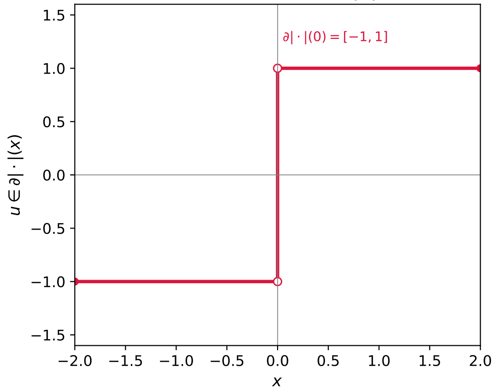
The multifunction x \mapsto \partial | \cdot |(x)
