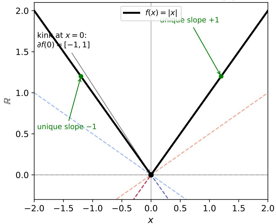
Supporting affine minorants of |x|
