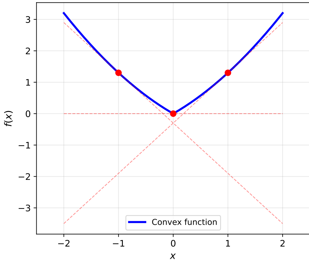
Convex Function: Supporting Hyperplanes
