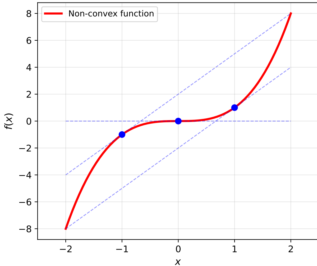
Non-convex: Tangents Not Supporting
