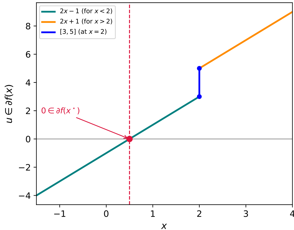
\partial f for f(x) = |x-2| + x^2
