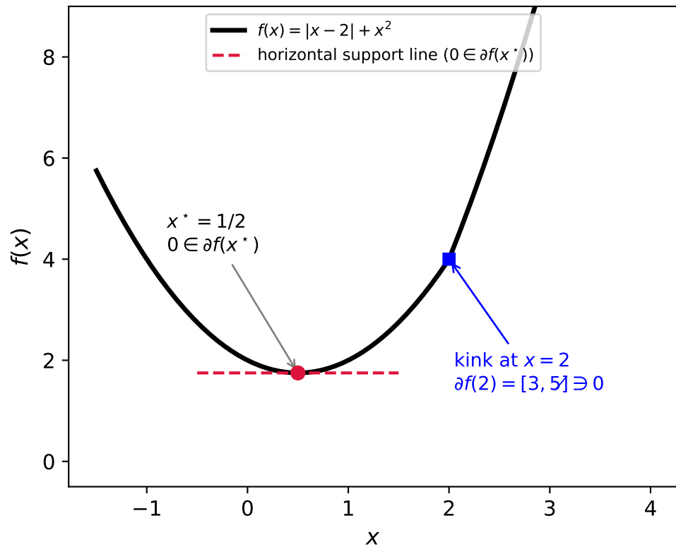
Fermat's rule: \text{Argmin } f = \text{zer } \partial f
