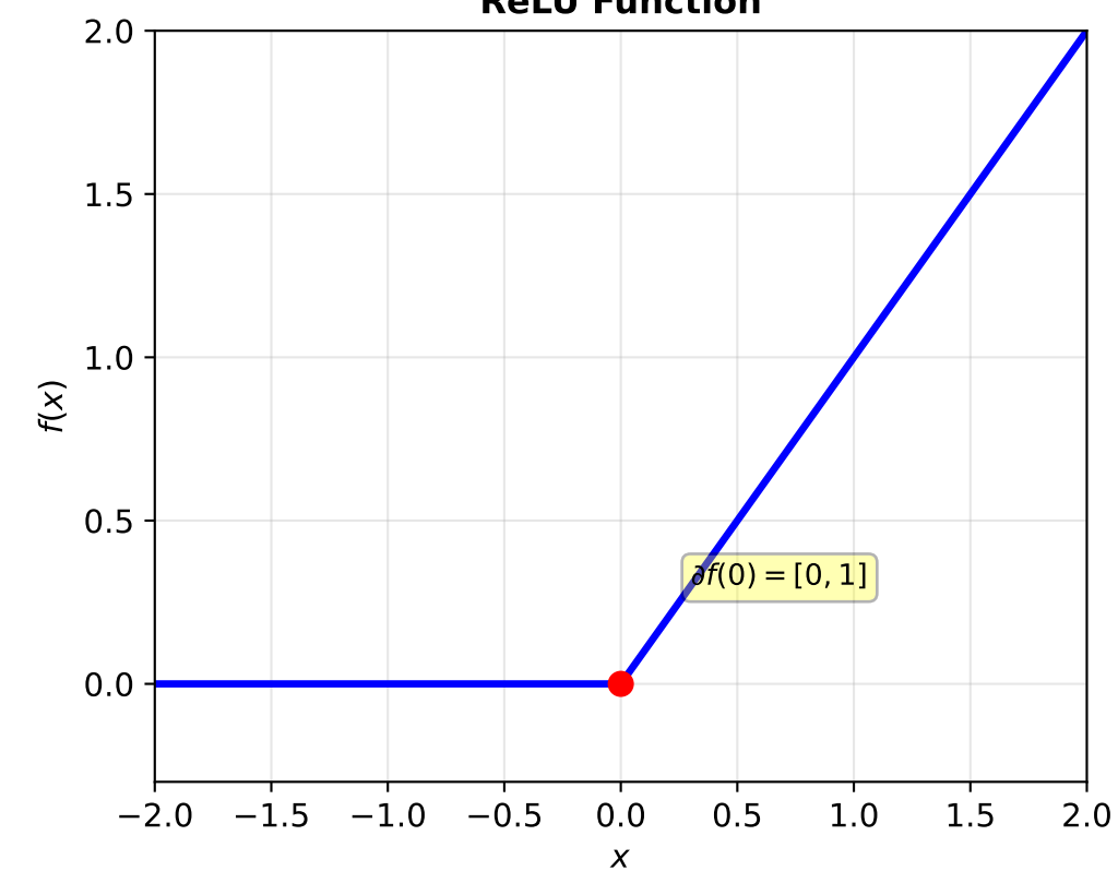
ReLU Function
