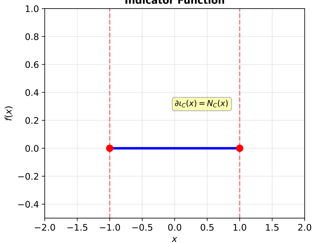
Indicator Function
