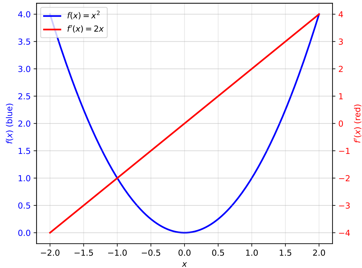
Convex Function and Monotone Gradient
