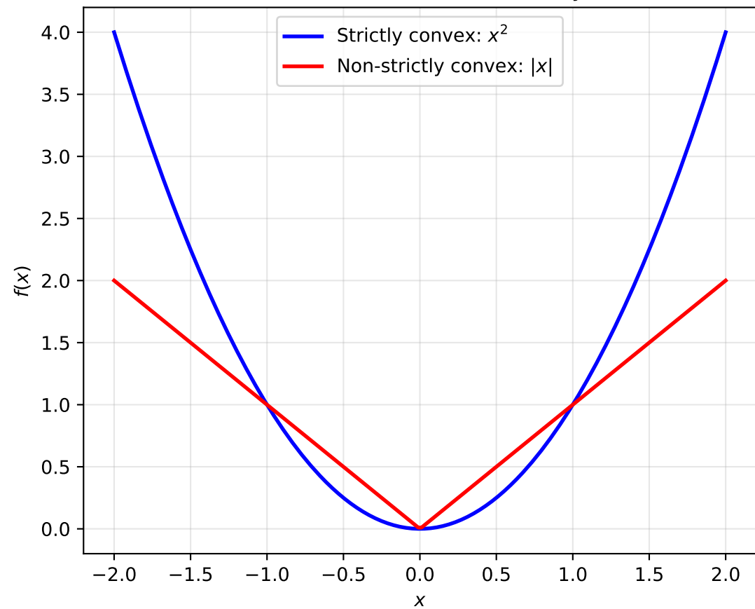
Strict vs Non-Strict Convexity
