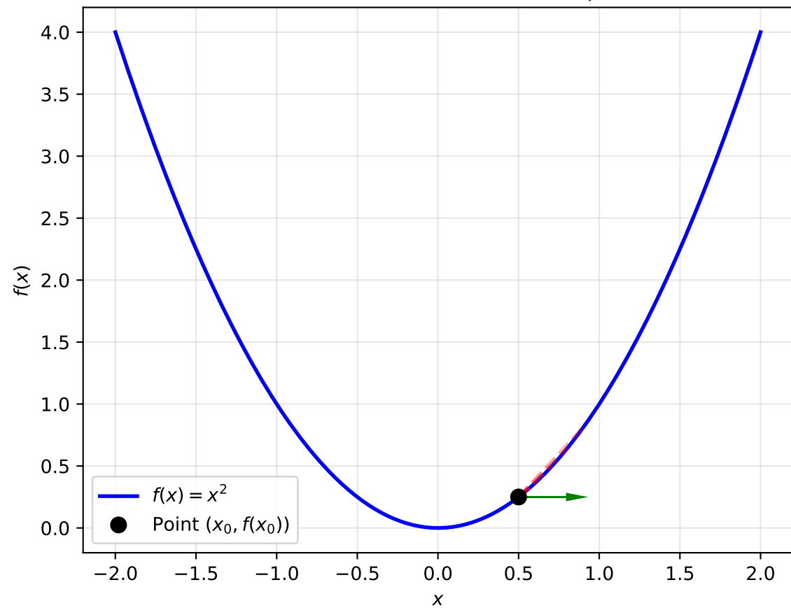
Directional Derivative Concept
