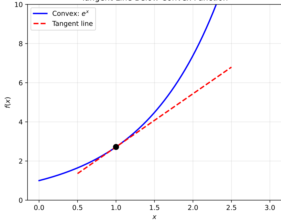
Tangent Line Below Convex Function
