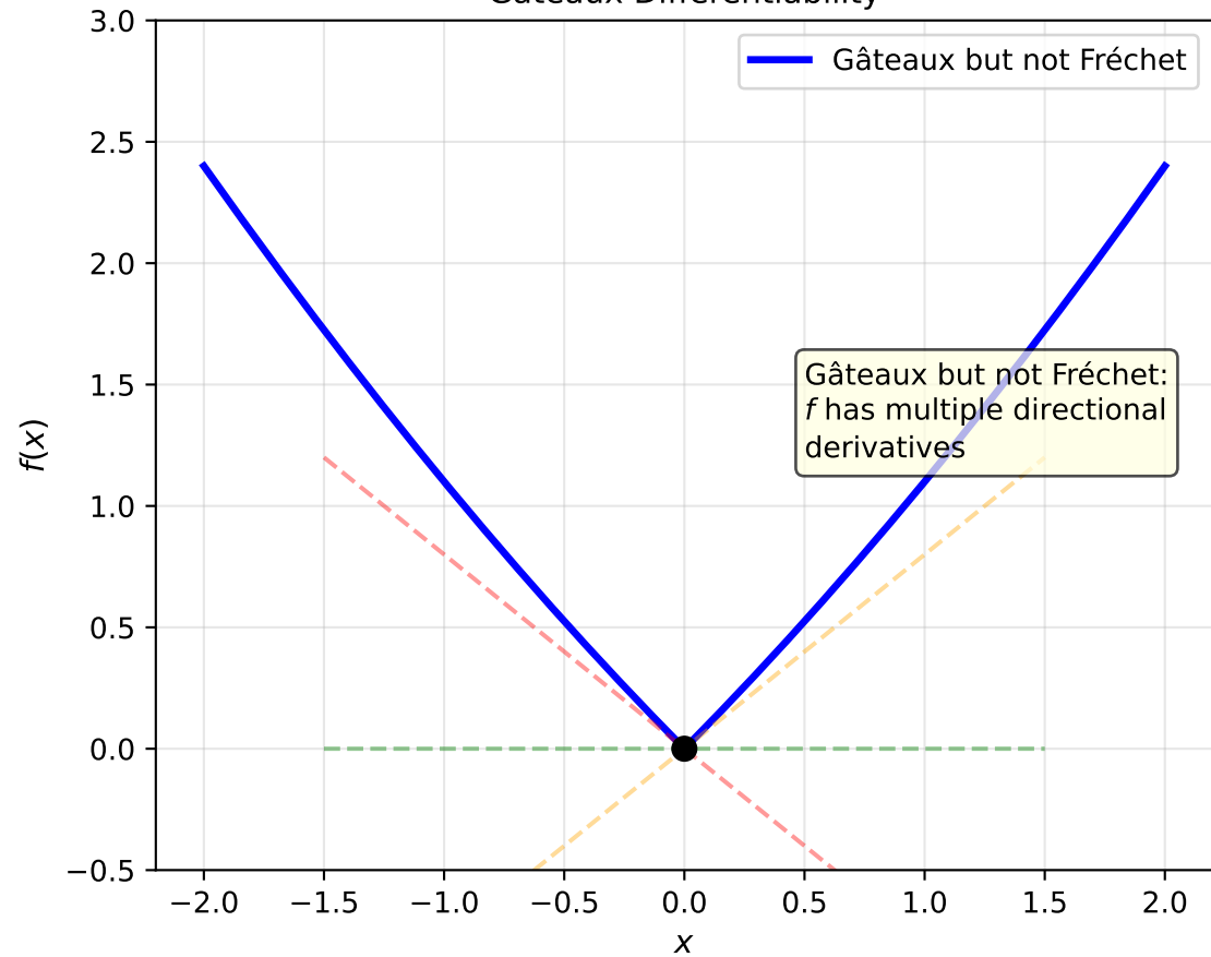
Gâteaux Differentiability
