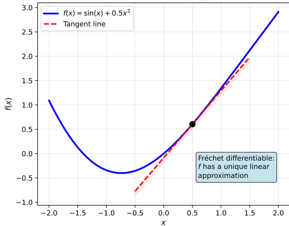
Fréchet Differentiability
