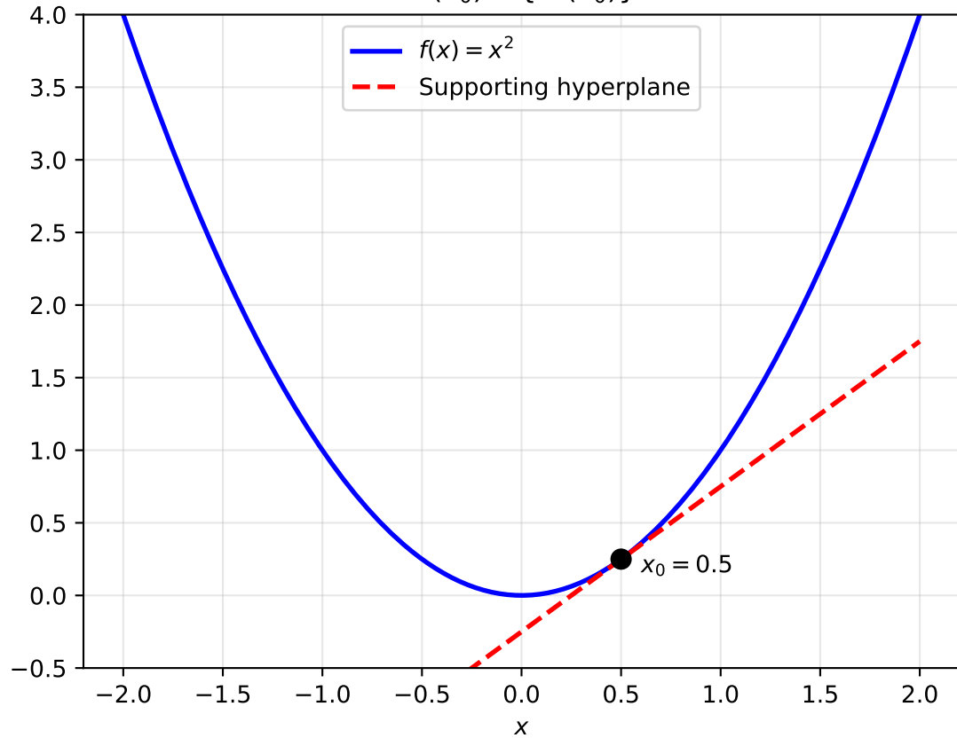
Subdifferential of Smooth Function
