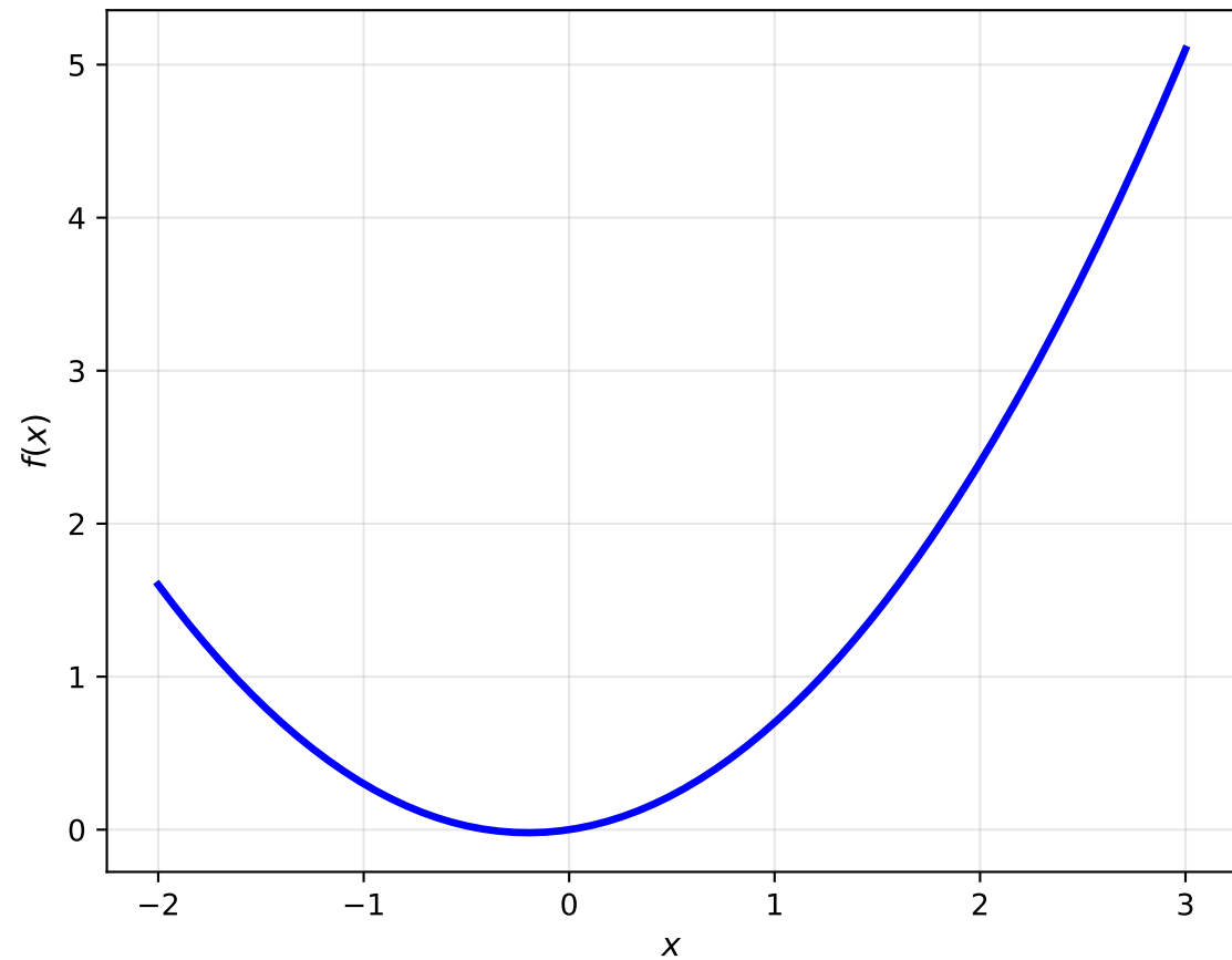
Function f with \beta -Lipschitz continuous gradient
