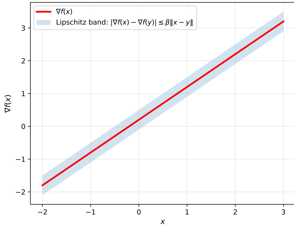
Gradient is Lipschitz continuous
