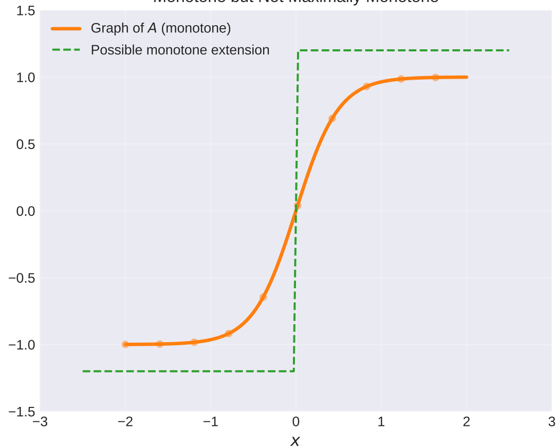
Monotone but Not Maximally Monotone
