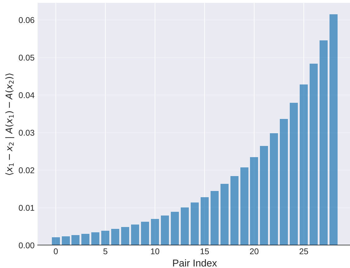
Monotonicity Check: \langle x - y \mid u - v \rangle \geq 0
