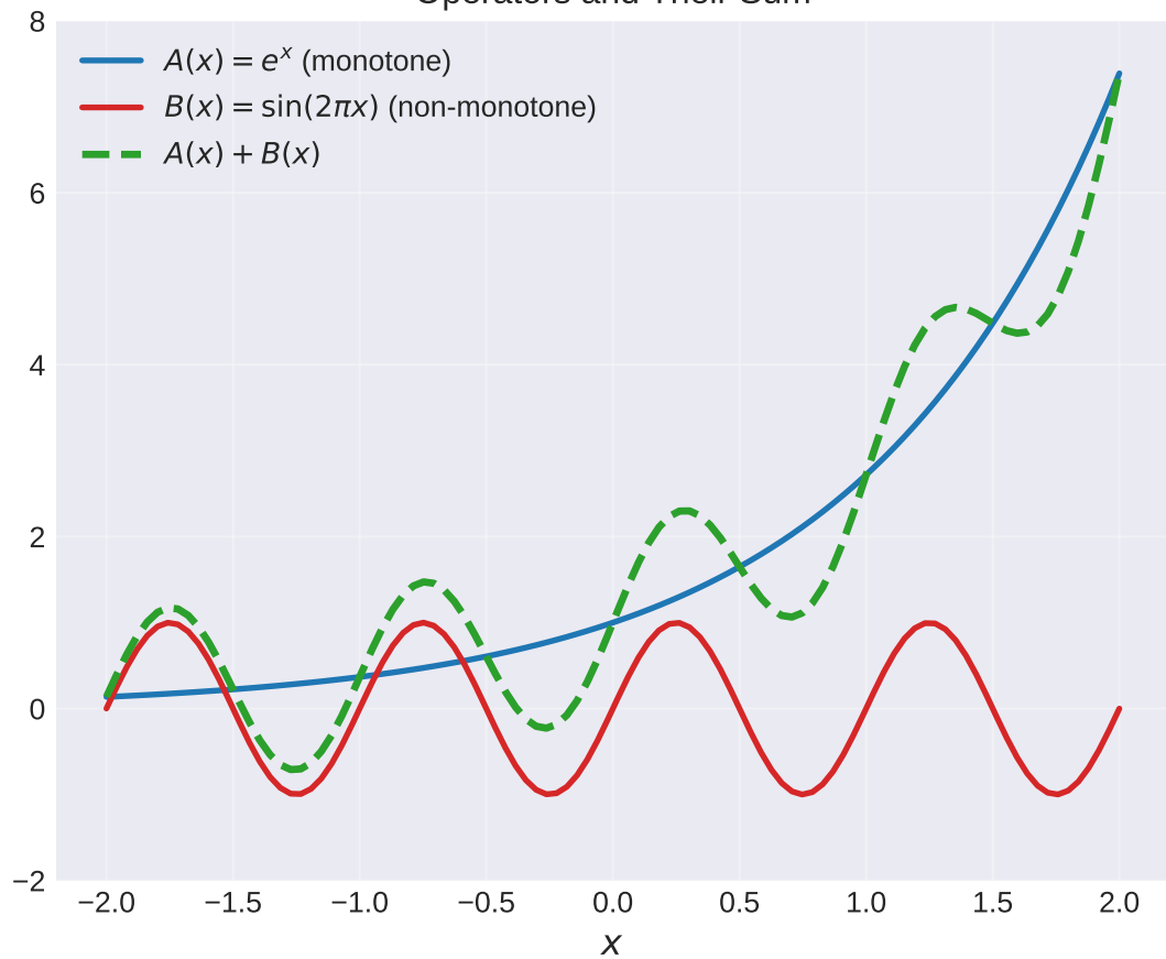
Operators and Their Sum
