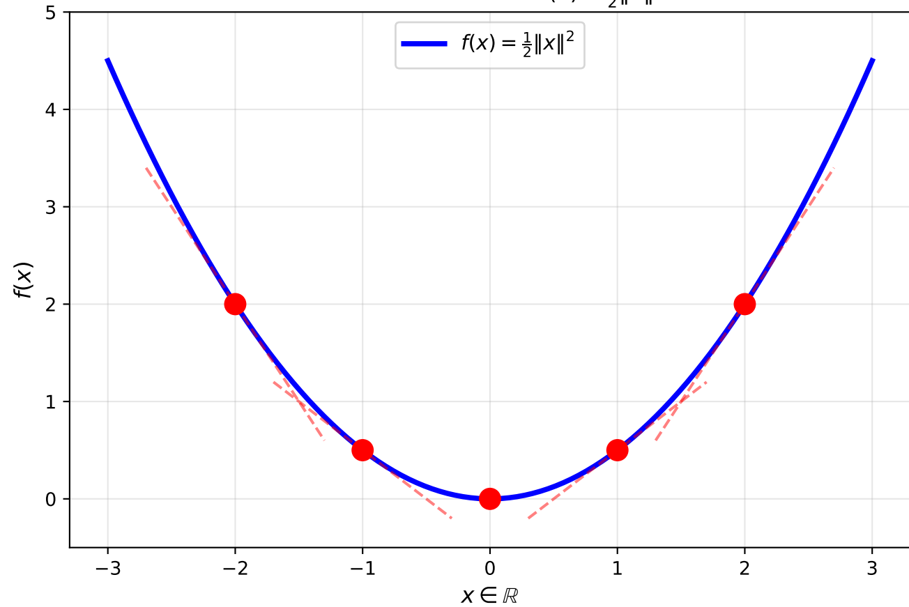
Convex Function: f(x) = \frac{1}{2}\|x\|^2
