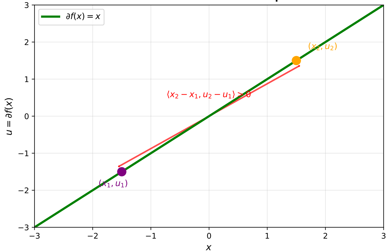
Subdifferential \partial f as Monotone Operator
