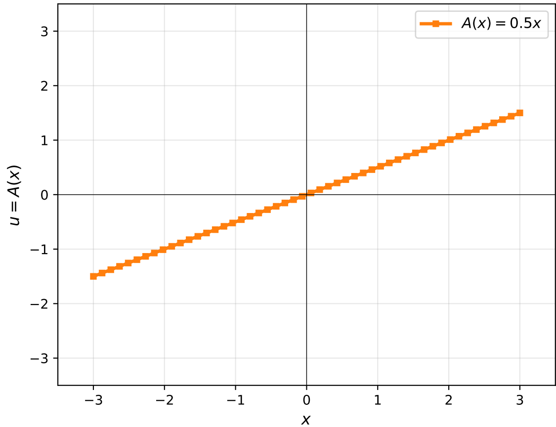
Monotone and Cocoercive: A(x) = 0.5x
