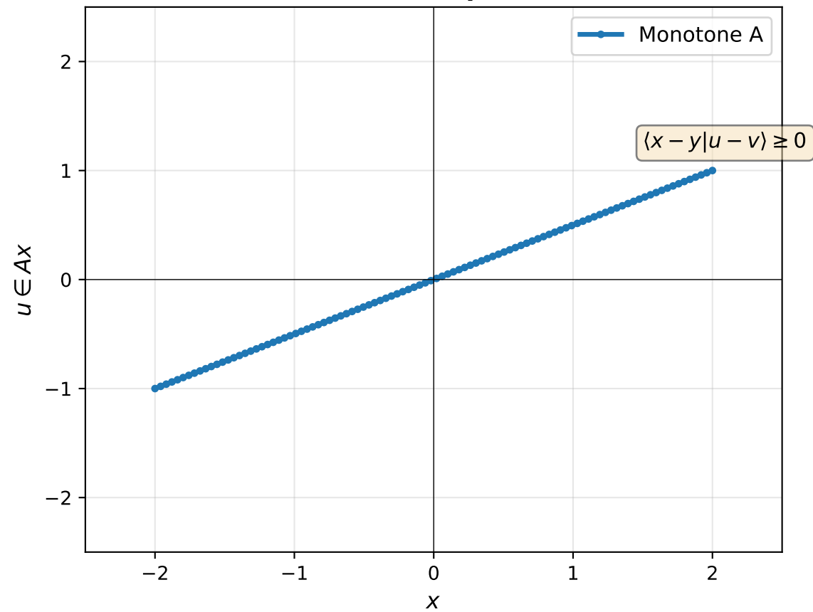
Monotone Operator
