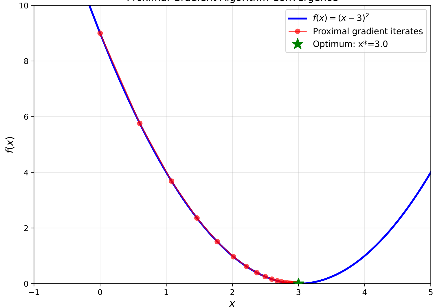
Proximal Gradient Algorithm Convergence
