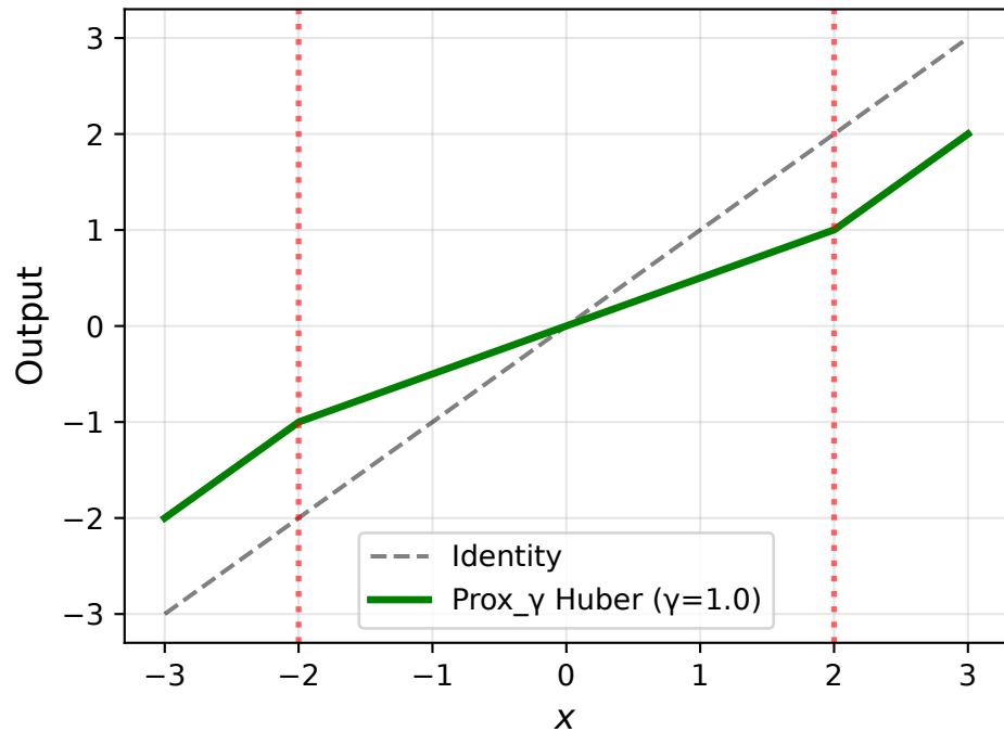
Proximal Operator of Huber
