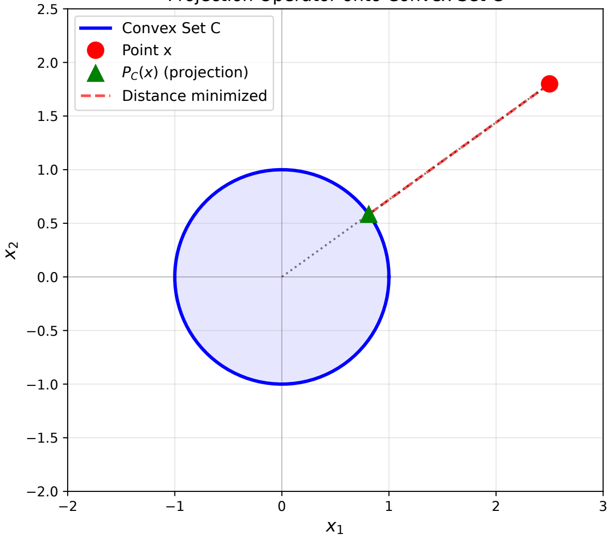
Projection Operator onto Convex Set C
