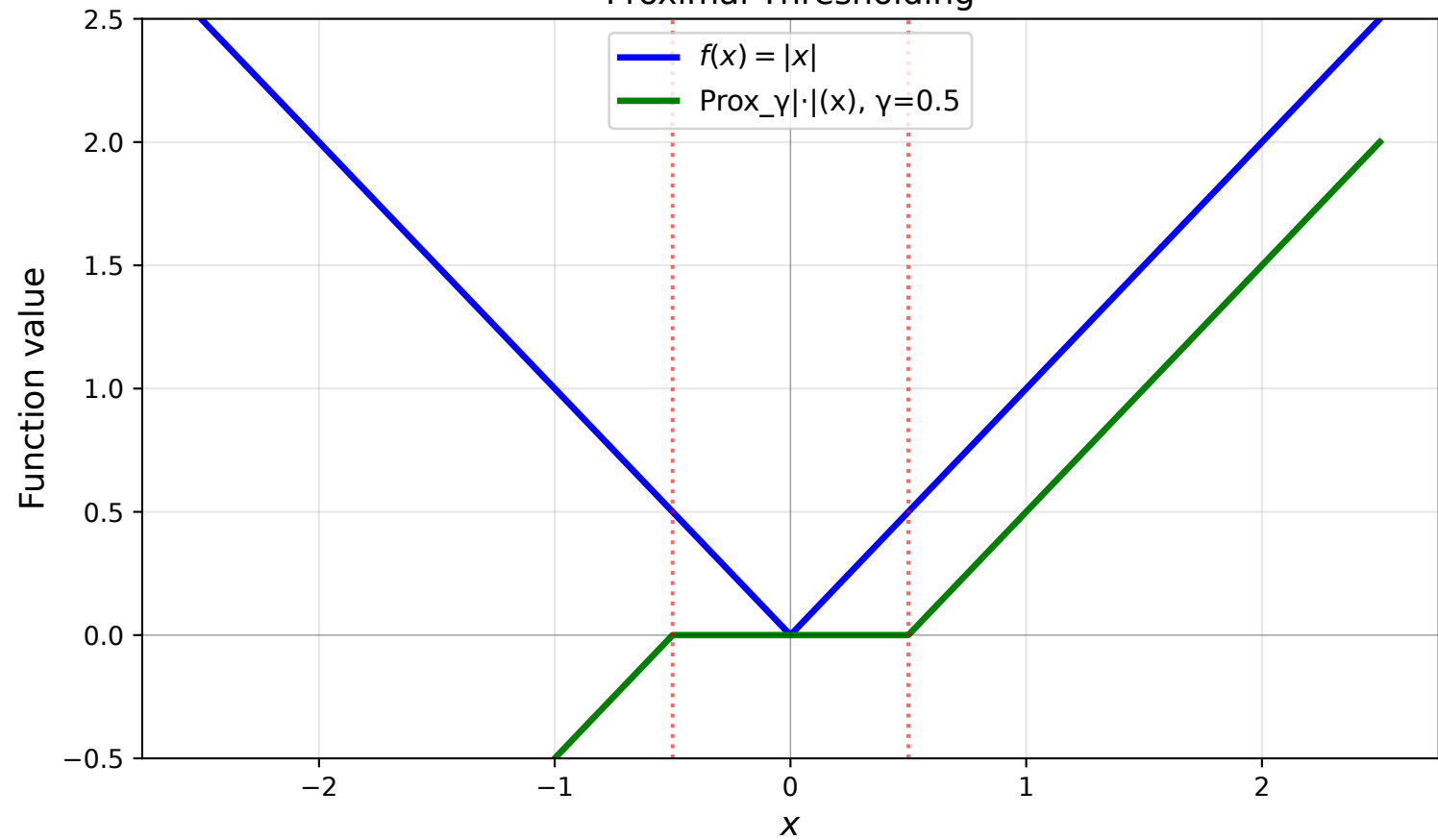
Proximal Thresholding
