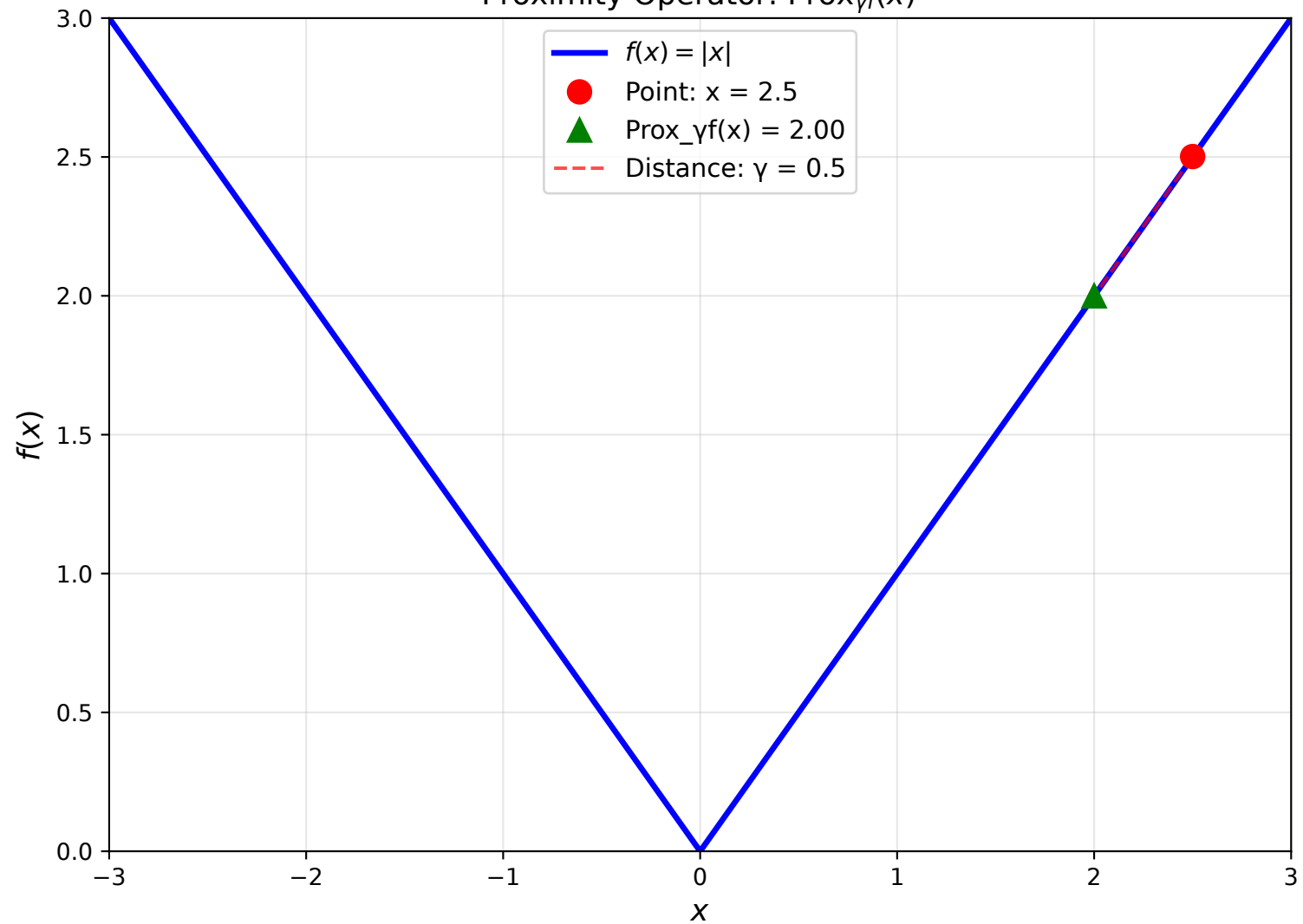
Proximity Operator: \text{Prox}_{\gamma f}(x)
