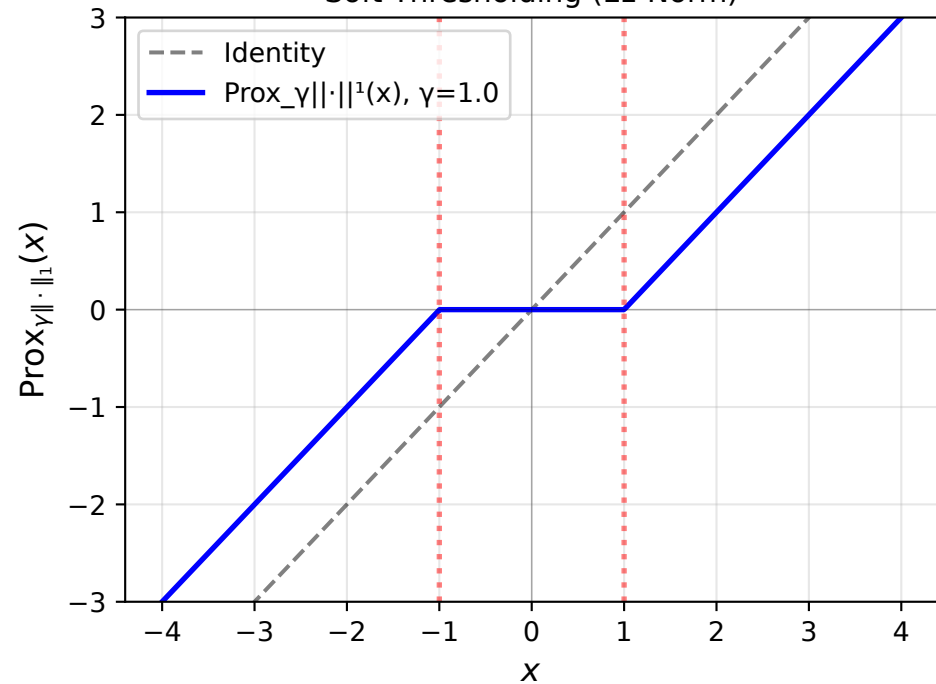
Soft Thresholding (L1 Norm)
