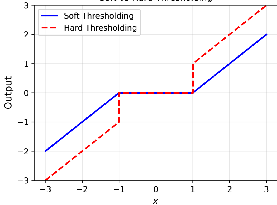
Soft vs Hard Thresholding
