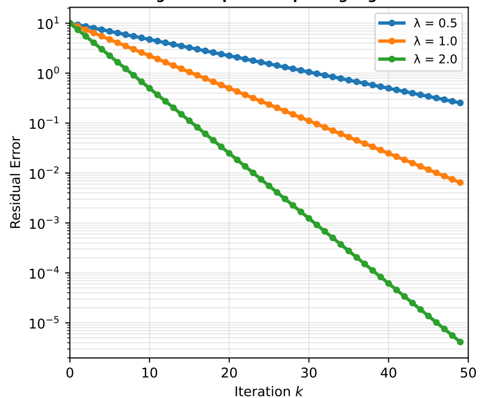
Convergence: Operator Splitting Algorithms
