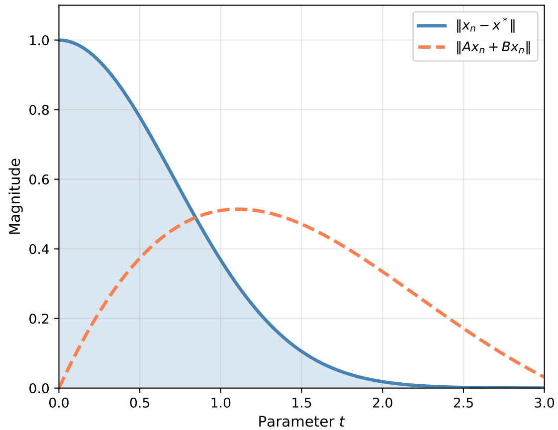
Solution Error vs Residual
