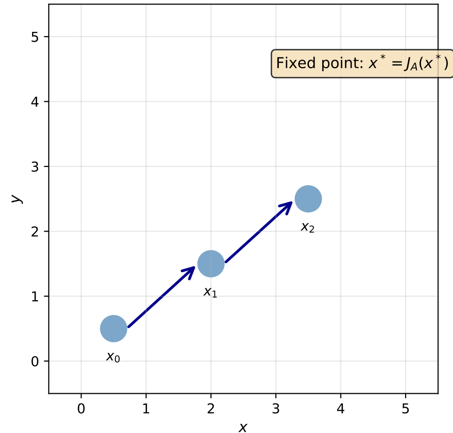
Resolvent Operator J_A = (\text{Id} + A)^{-1}
