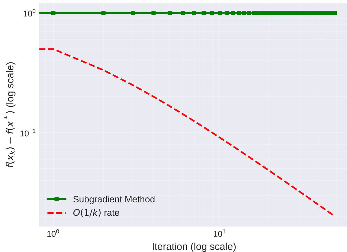
Sublinear Convergence (Non-smooth)
