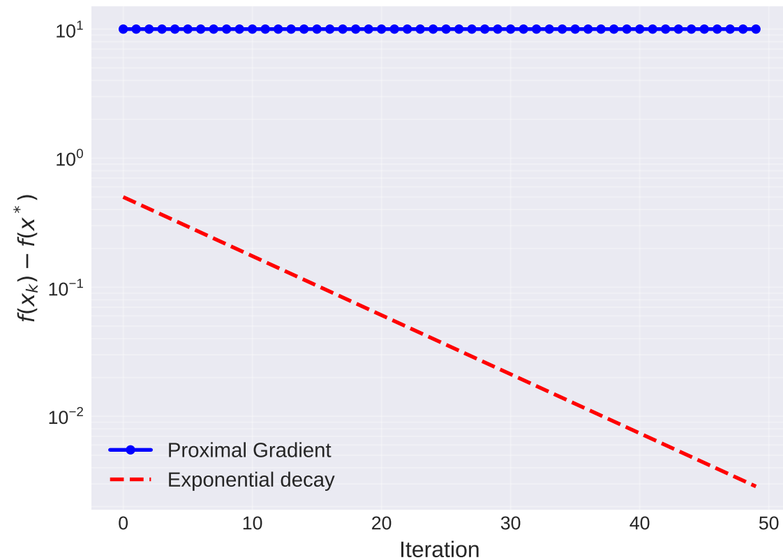
Linear Convergence (Smooth + Strongly Convex)
