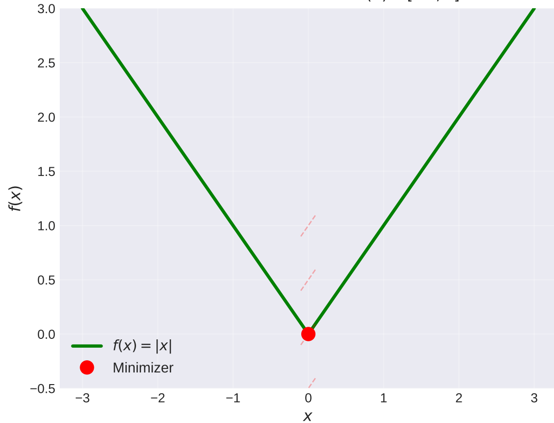
Non-smooth function: 0 \in \partial f(0) = [-1, 1]
