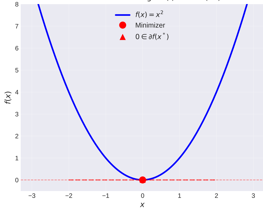
Fermat's Rule: x^* \in \text{Argmin}(f) \Leftrightarrow 0 \in \partial f(x^*)
