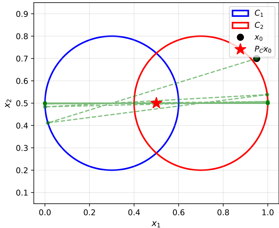
Dykstra's Algorithm: Projection onto C_1 \cap C_2
