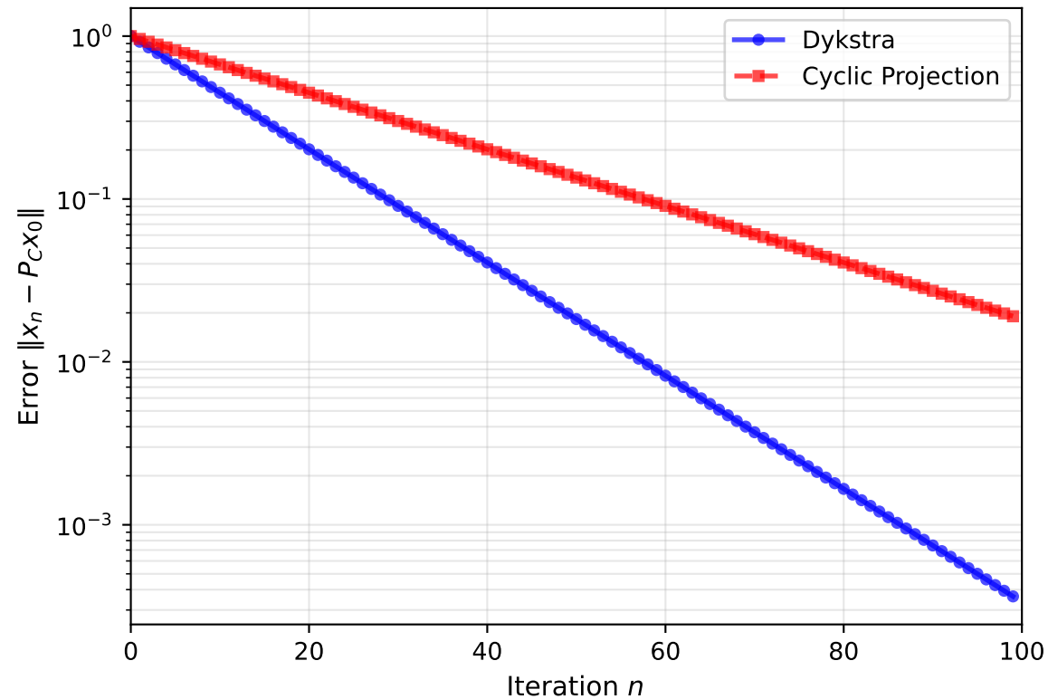
Dykstra vs. Cyclic Projection
