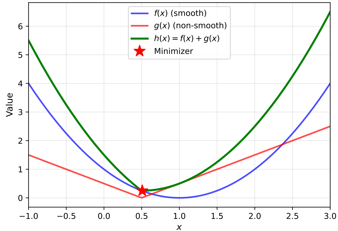
Forward-Backward: Problem Setup
