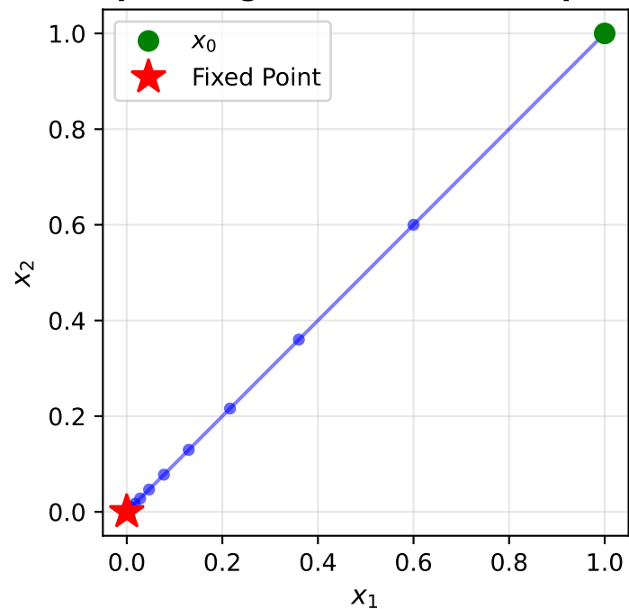
Halper's Algorithm: Iterate Sequence
