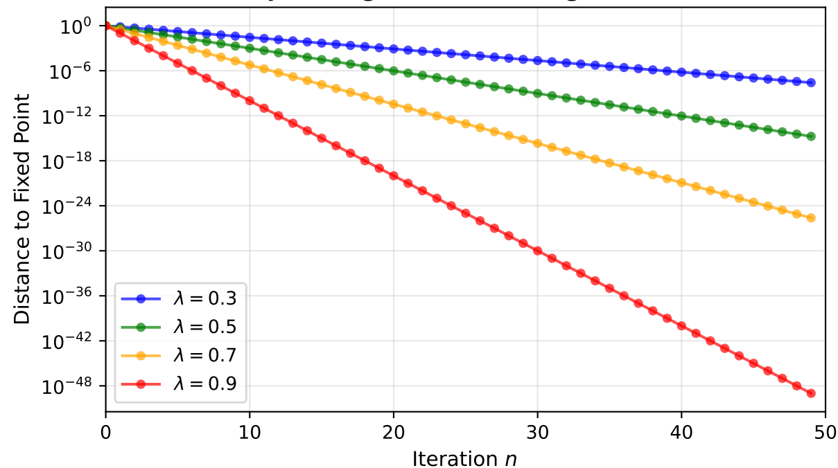
Halper's Algorithm: Convergence Rate
