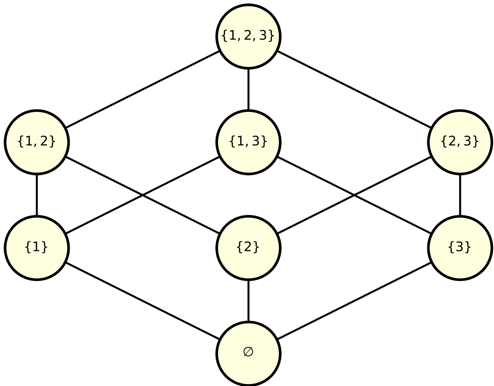
Boolean Lattice B_3 (Power Set of \{1, 2, 3\} )
