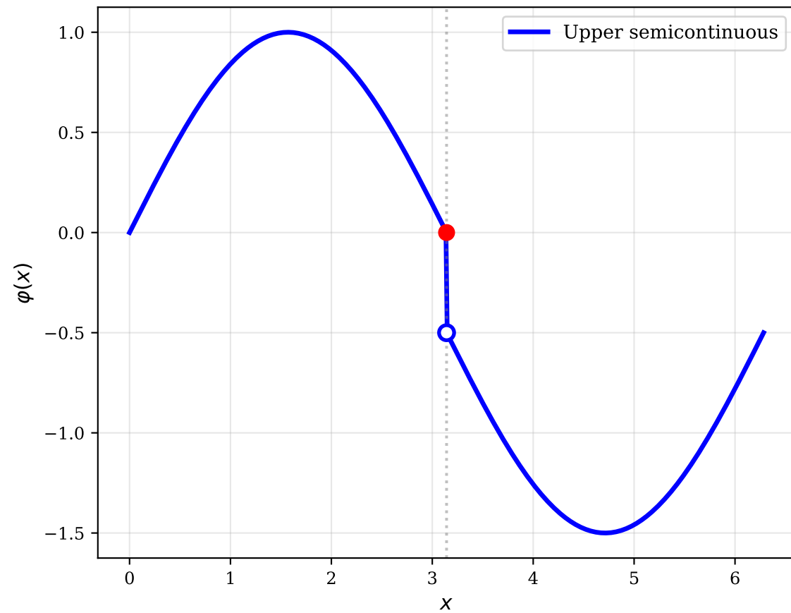
Upper Semicontinuous at x_0 = \pi
