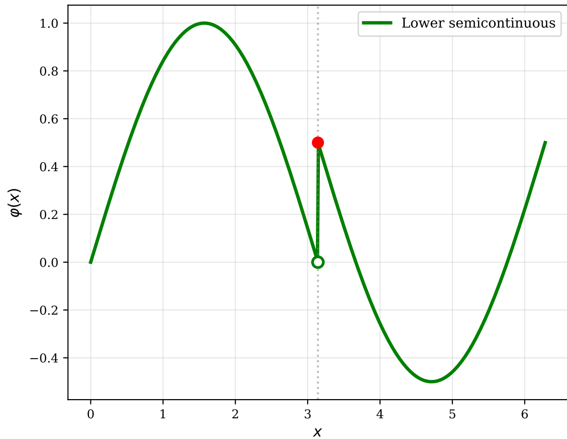
Lower Semicontinuous at x_0 = \pi
