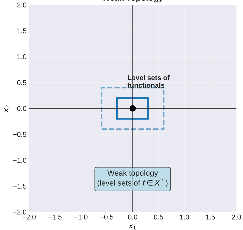
Weak Topology
