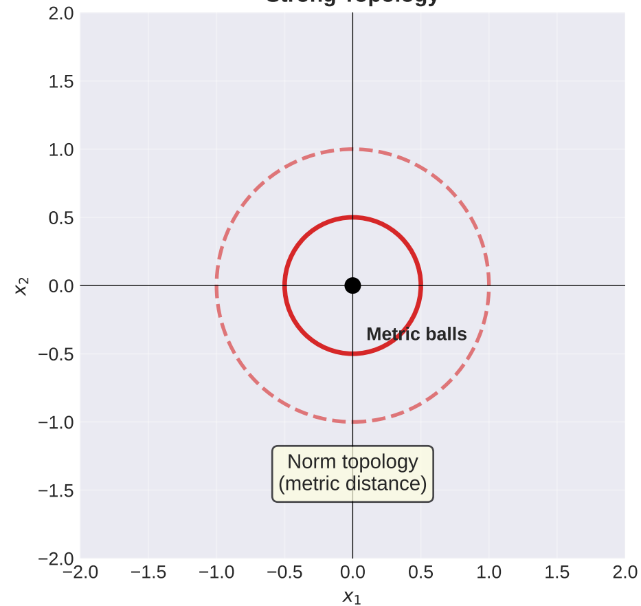
Strong Topology
