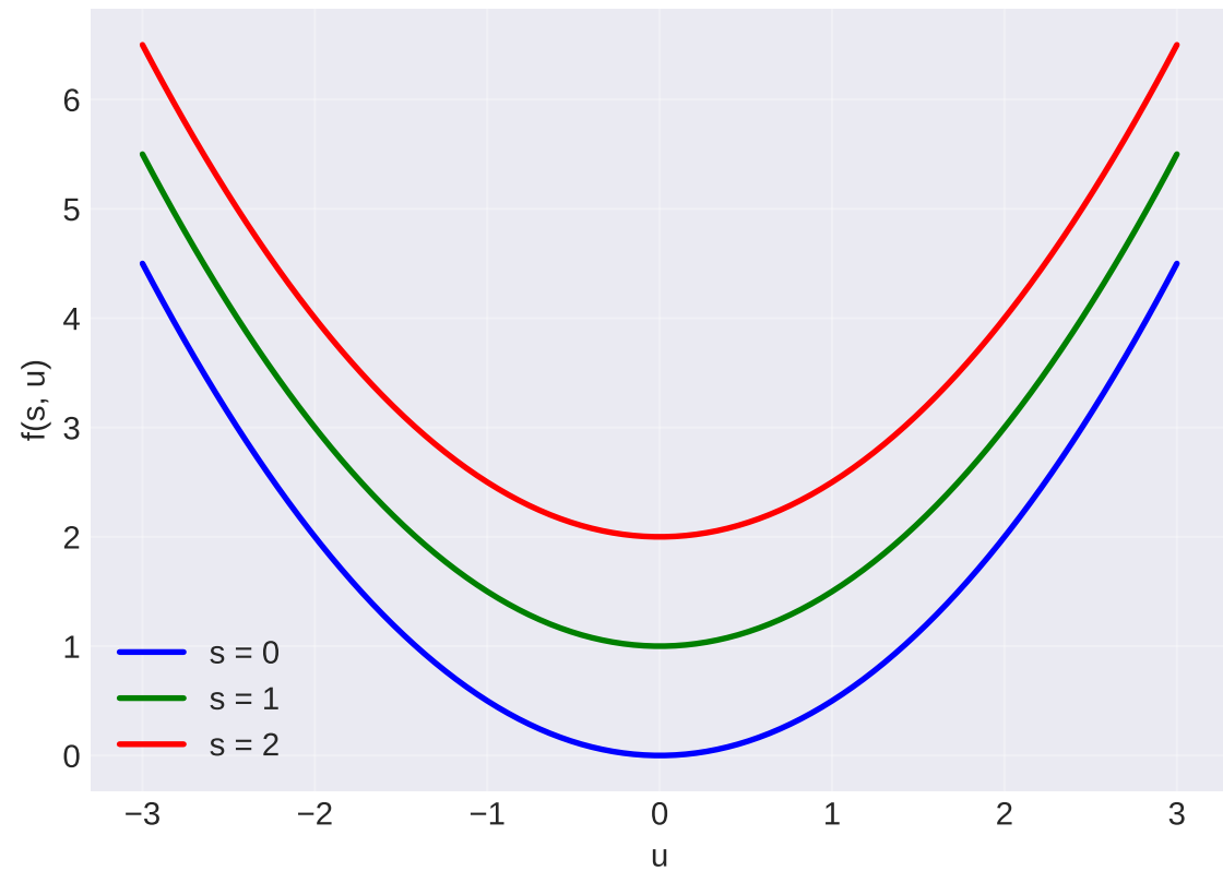
Function f(s, u) for different s
