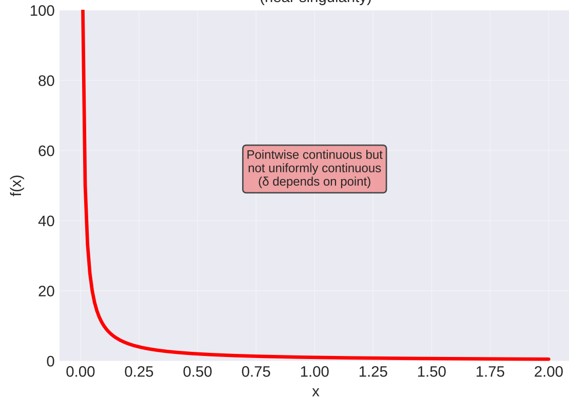
Non-Uniformly Continuous Function (near singularity)
