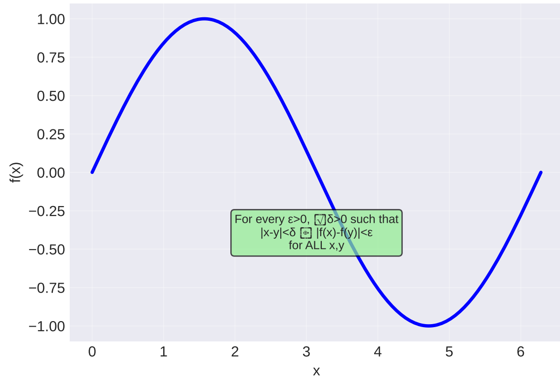
Uniformly Continuous Function (on compact set)
