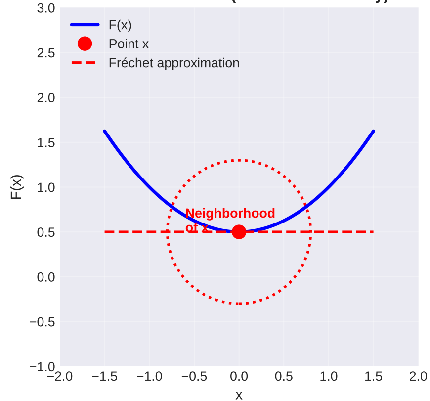
Fréchet Derivative (Full Differentiability)
