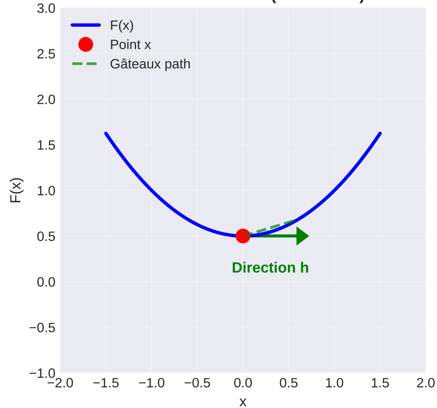
Gâteaux Derivative (Directional)
