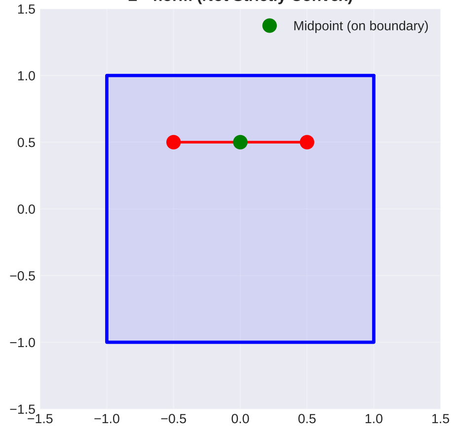
L^\infty norm (Not Strictly Convex)
