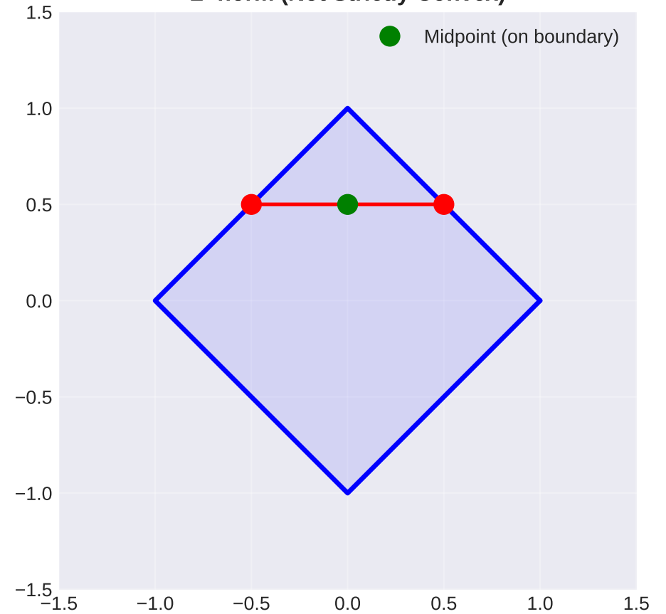
L^1 norm (Not Strictly Convex)
