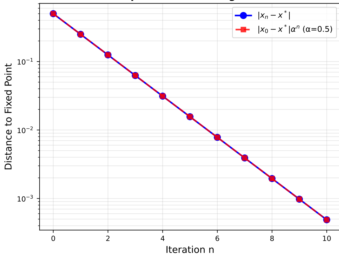
Exponential Convergence
