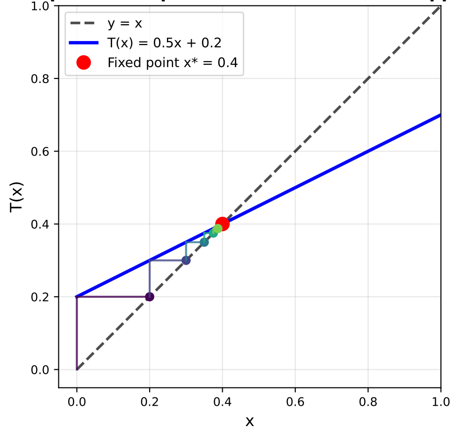
Graphical Interpretation of Contraction Mapping
