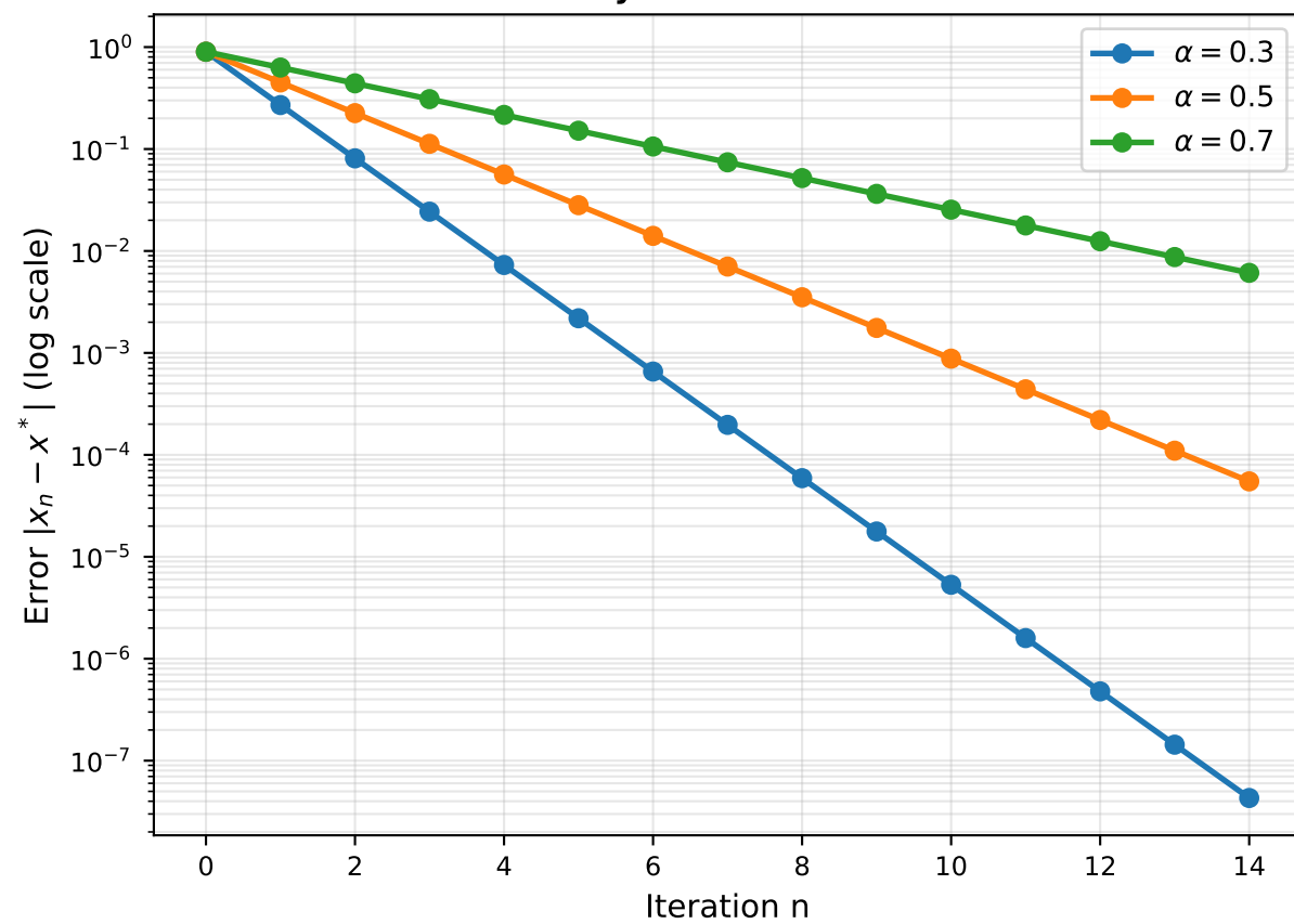
Error Decay for Different \alpha Values
