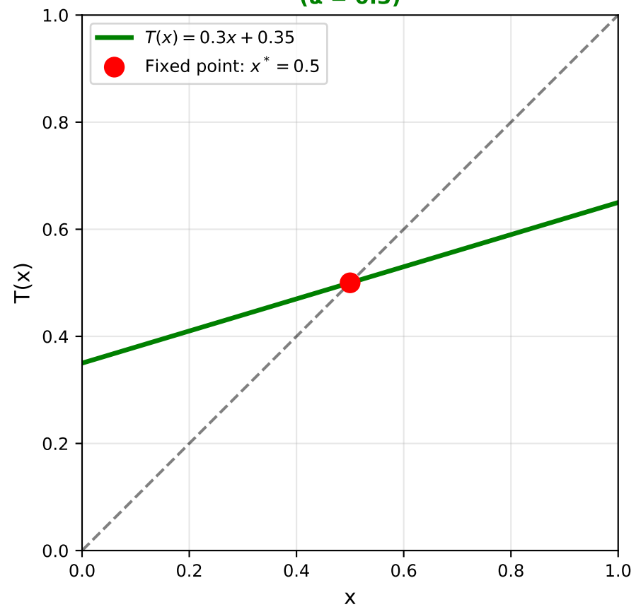
✓ Stronger Contraction ( \alpha = 0.3 )
