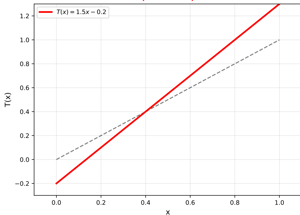
✗ Not a Contraction ( \alpha = 1.5 > 1 )
