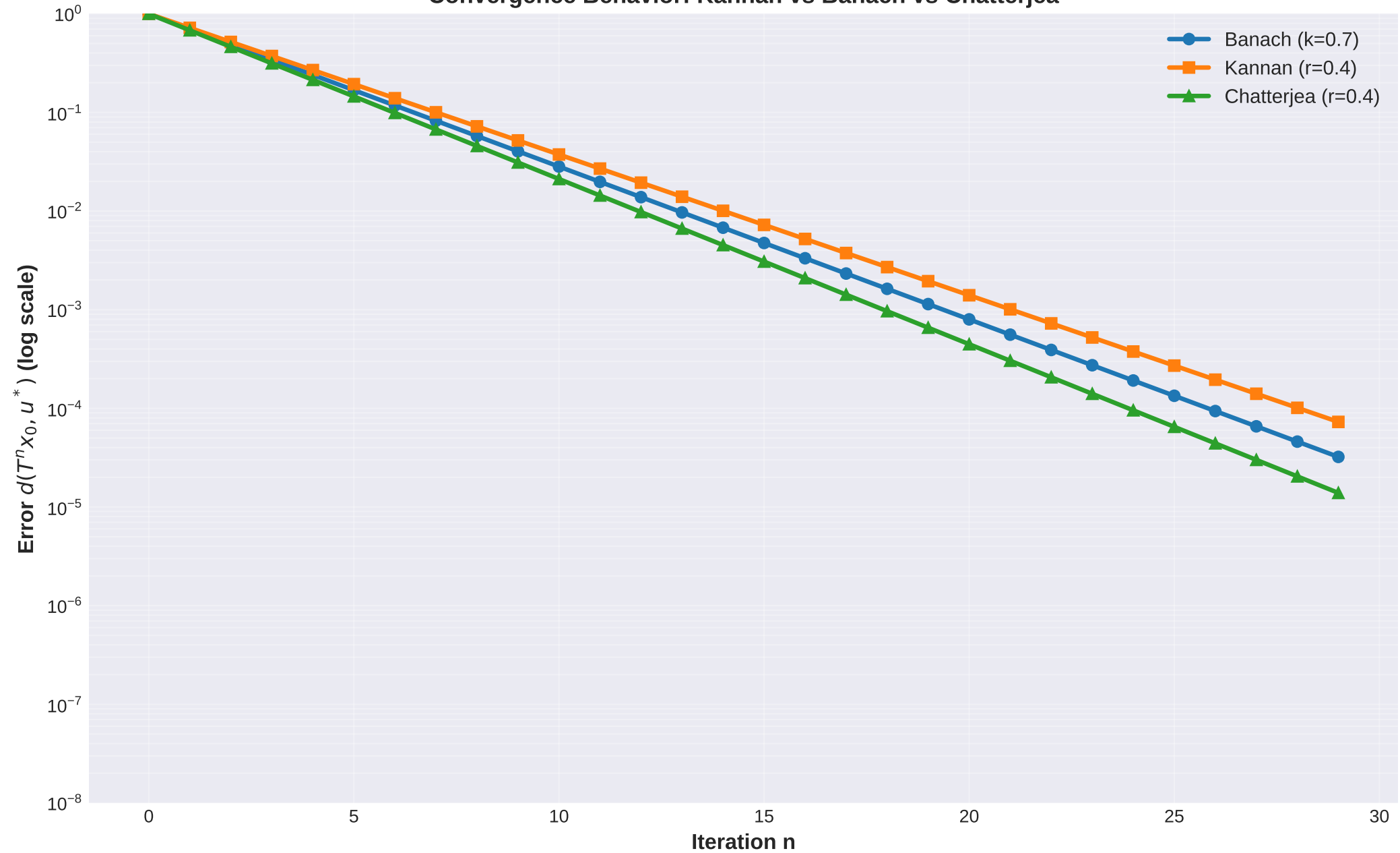
Convergence Behavior: Kannan vs Banach vs Chatterjea
