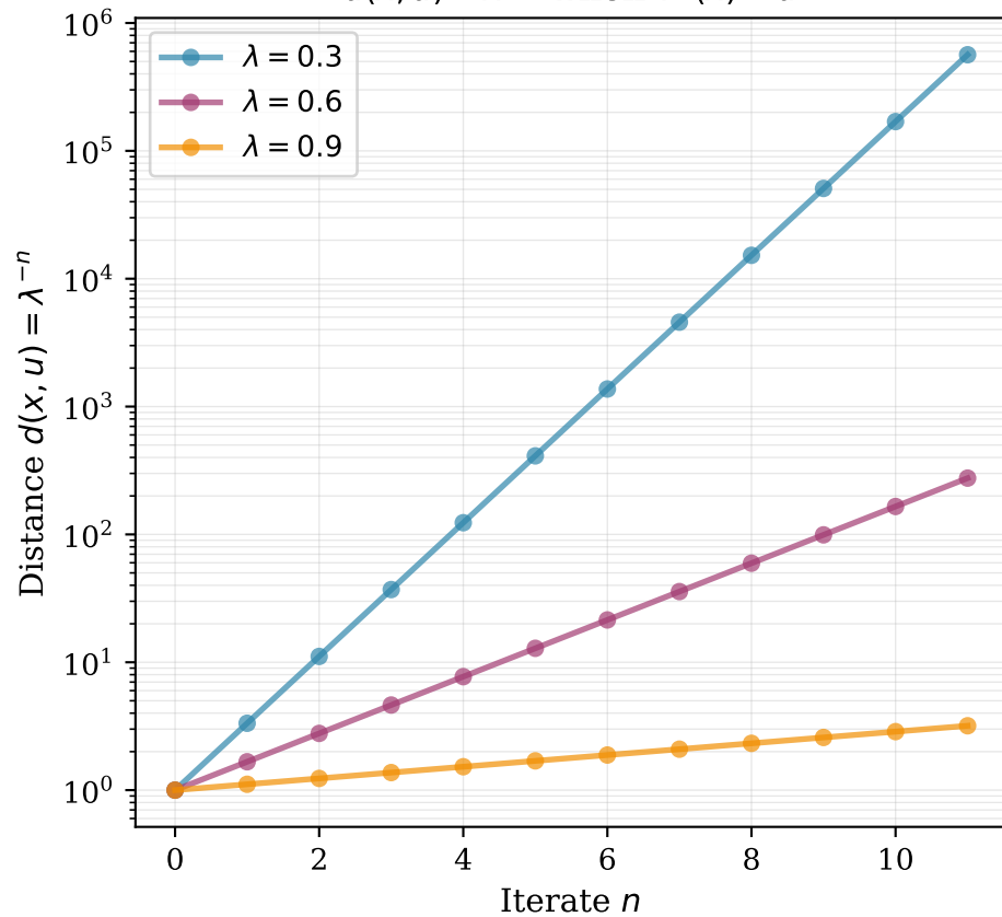
Metric Construction in Bessaga Theorem
