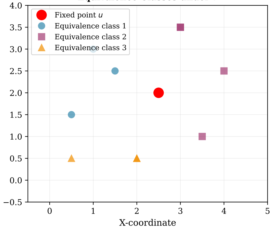
Bessaga's Converse Equivalence Classes under T
