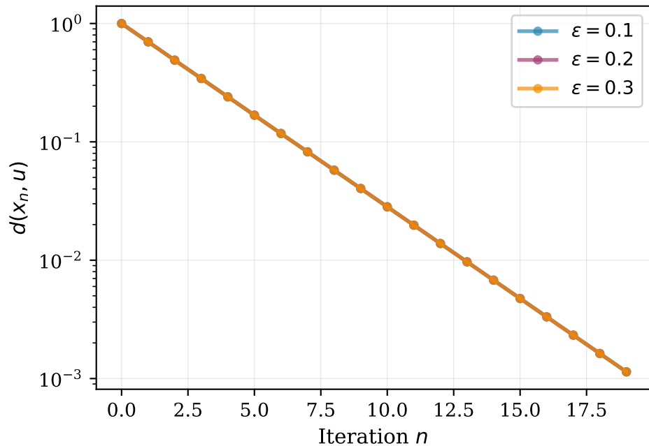
Edelstein Theorem \varepsilon -local Contraction Convergence
