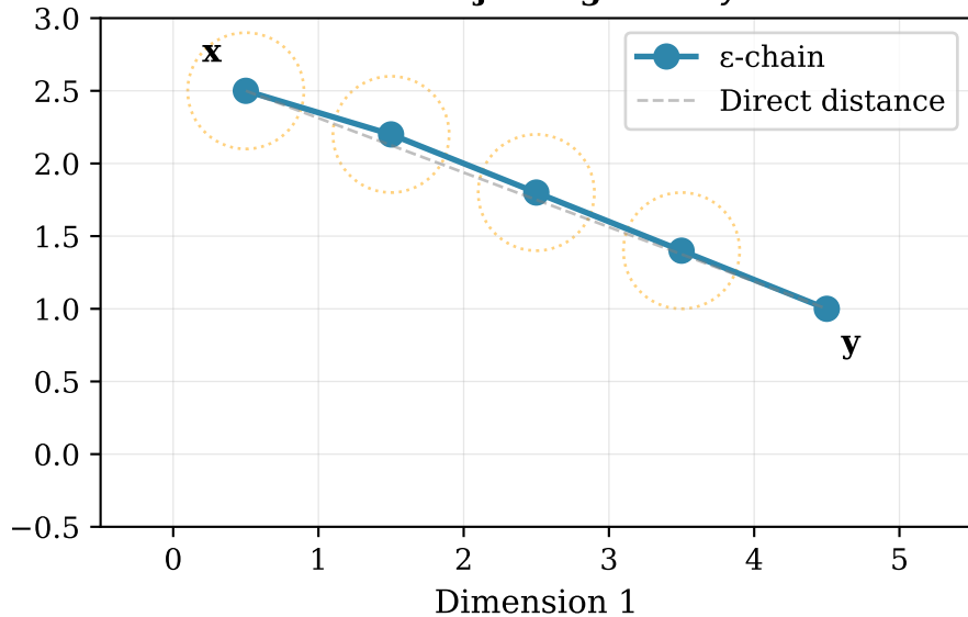
\varepsilon -Chainable Metric Space \varepsilon -chain joining x and y
