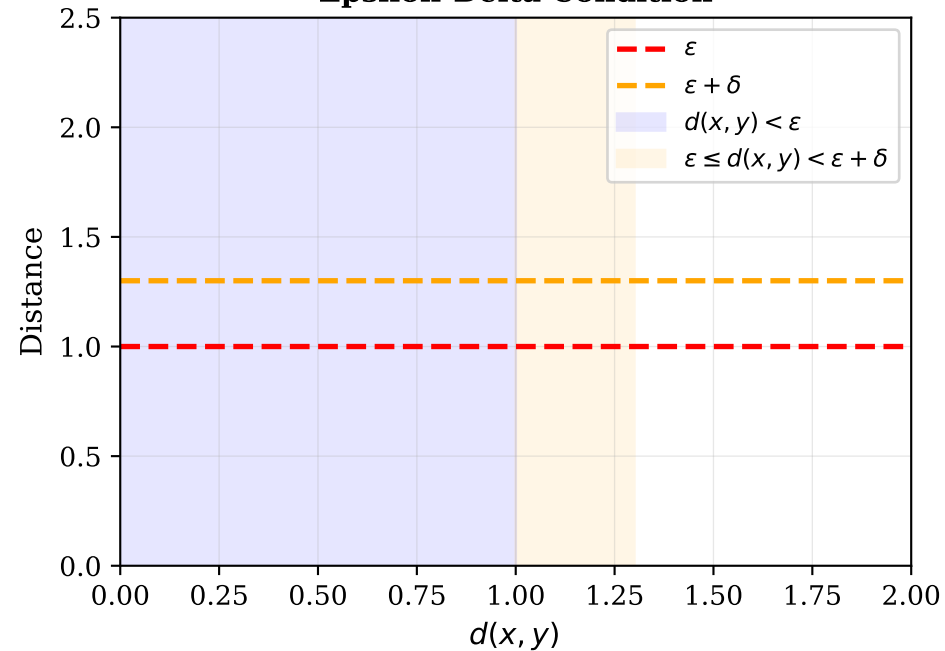
Meir-Keeler Contraction Epsilon-Delta Condition
