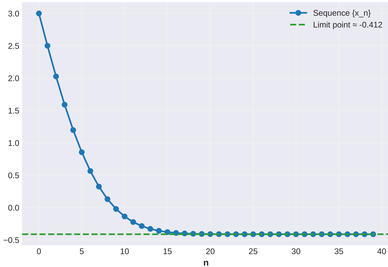
Generalized Nonexpansive Sequence
