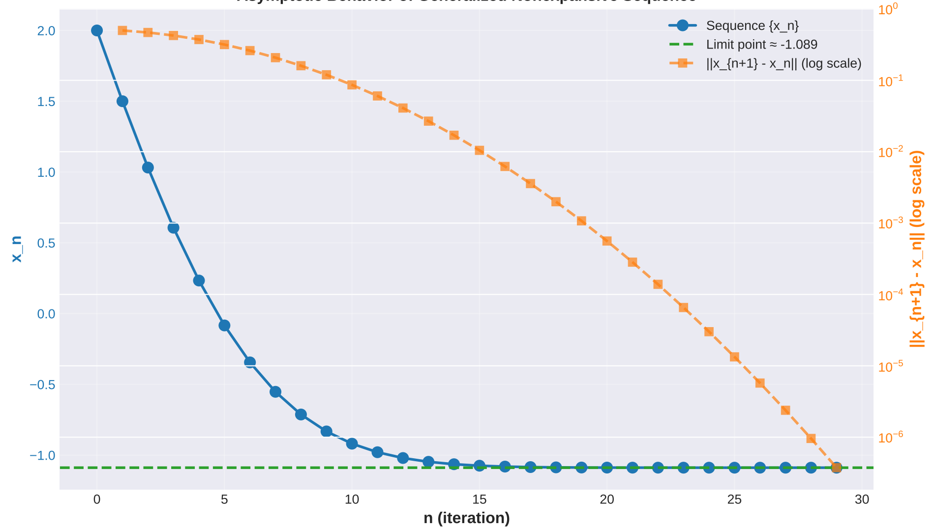
Asymptotic Behavior of Generalized Nonexpansive Sequence
