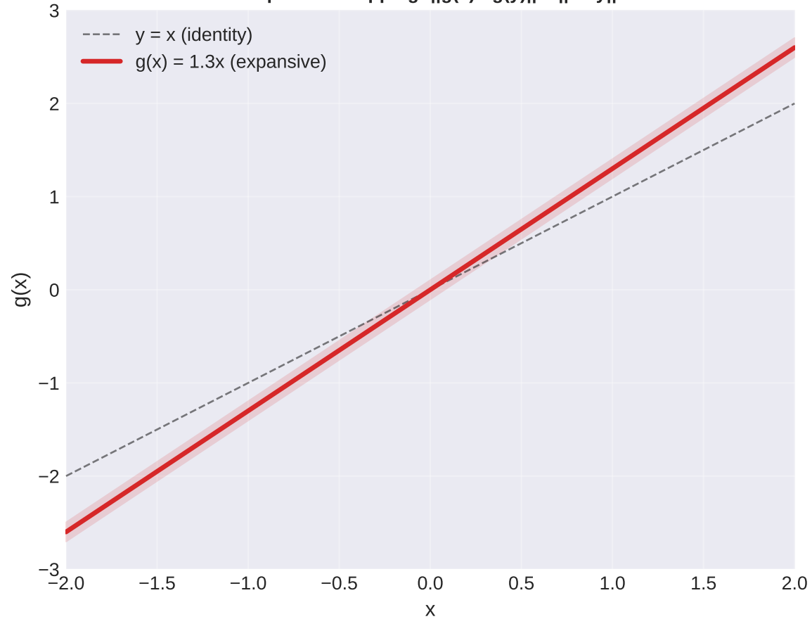
Expansive Mapping: \|g(x) - g(y)\| > \|x - y\|
