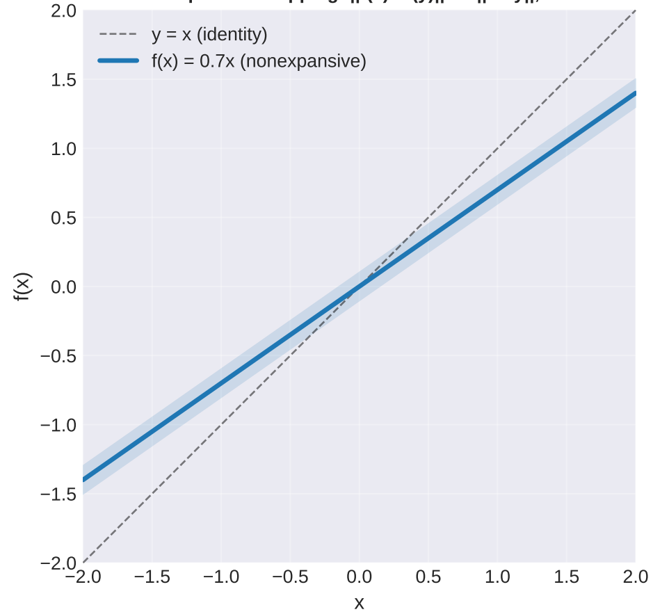
Nonexpansive Mapping: \|f(x) - f(y)\| \leq L\|x - y\| , L < 1
