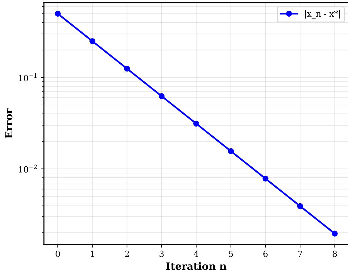
Convergence: Error vs Iteration
