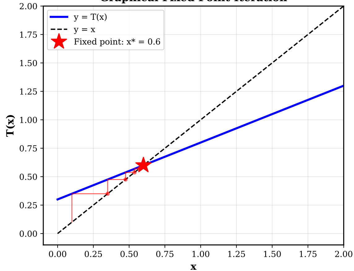
Graphical Fixed Point Iteration
