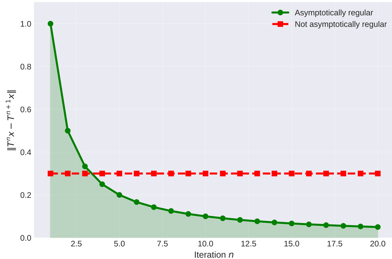
Asymptotic Regularity: \|T^n x - T^{n+1} x\| \rightarrow 0 as n \rightarrow \infty
