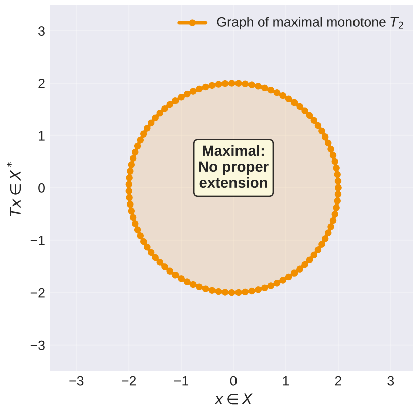
Maximal Monotone
