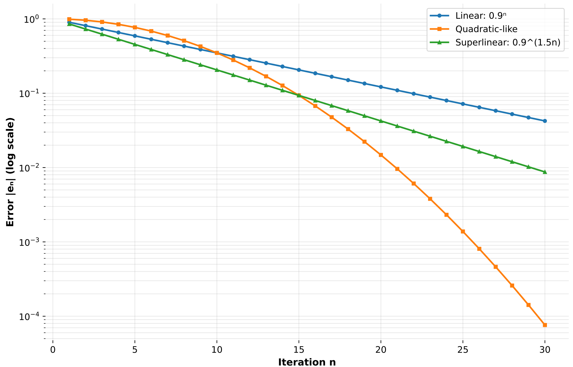
Convergence Rates Comparison
