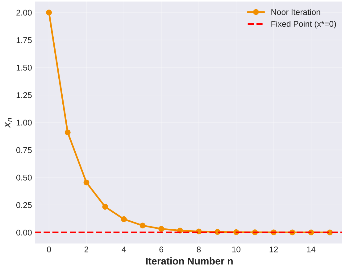
Noor Iteration Convergence: T(x) = 0.5\sin(x)
