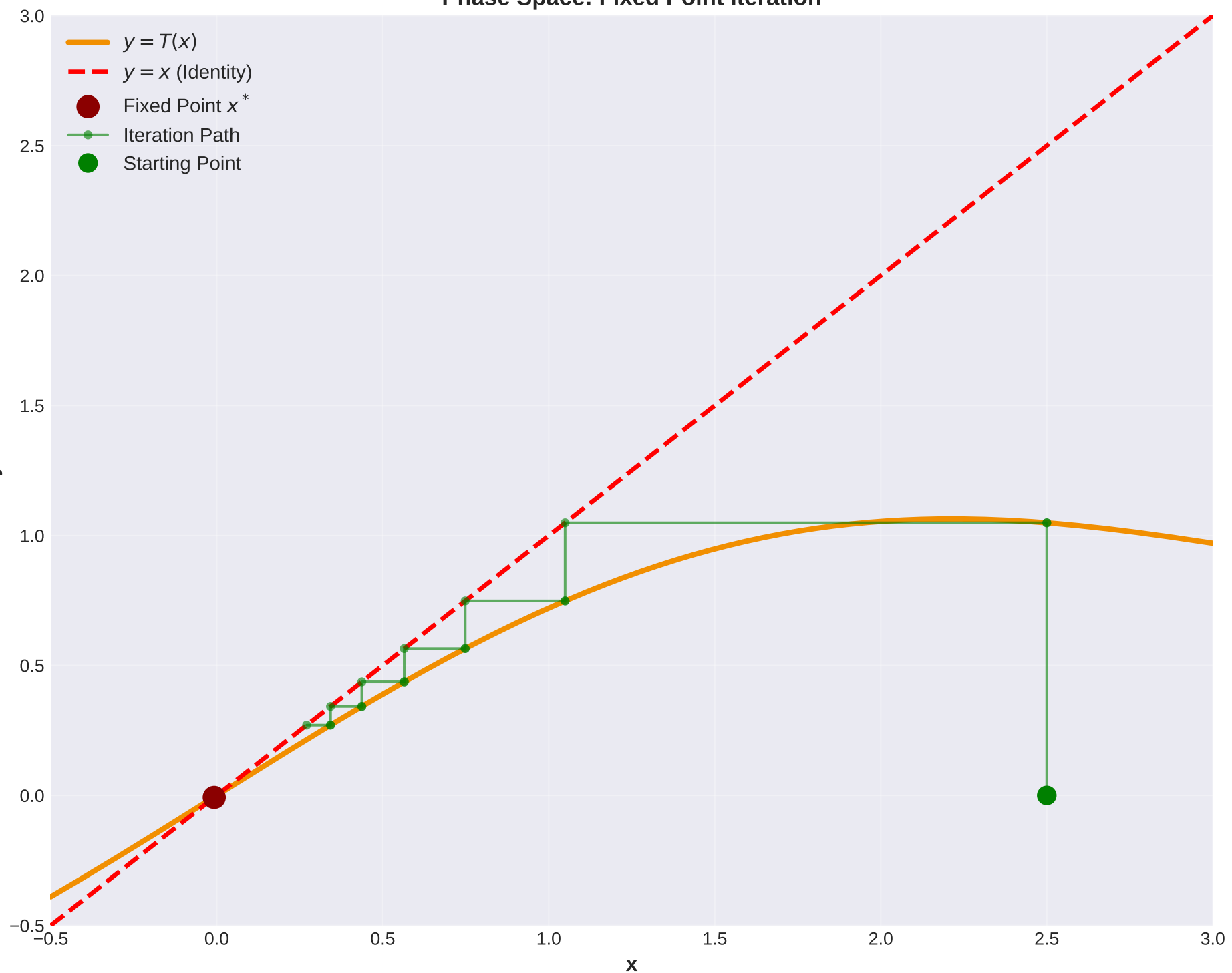
Phase Space: Fixed Point Iteration
